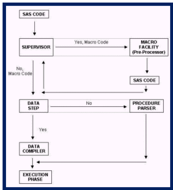
Figure 1: Macro Program Control Flow.
